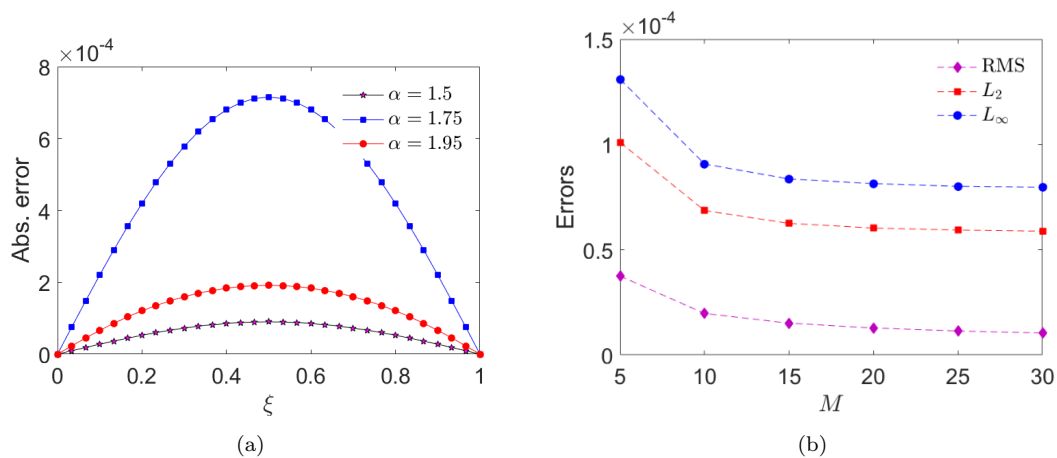
FIGURE 6. The 2D errors graph with (a) M = 30 , \Delta\tau = 0 , and \alpha = 1.5 , 1.75 , and 1.95 (b) \alpha = 1.95 and \Delta\tau = 0.005 at \tau = 1 for Example 6.2.
