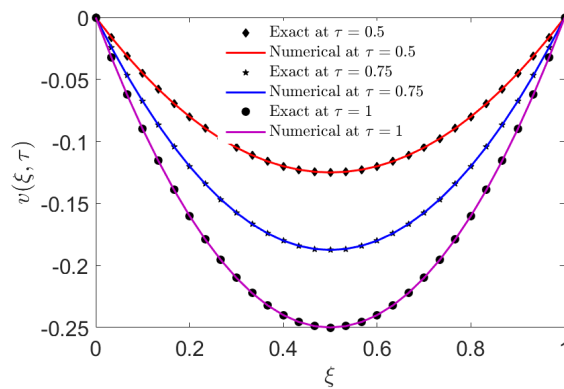
FIGURE 5. The exact and numerical v(\xi, \tau) with \alpha=1.95 , M=15 , \Delta\tau=0.001 at \tau=0.5 , 0.75 , and 1 for Example 6.2.
