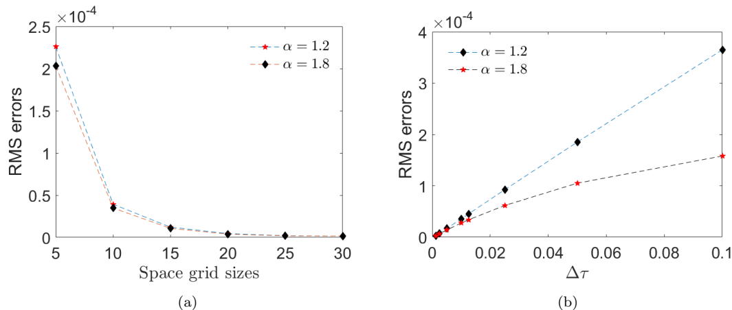
FIGURE 2. The RMS error norms vs. space grid size (a) and time grid size (b) for Example 6.1.
