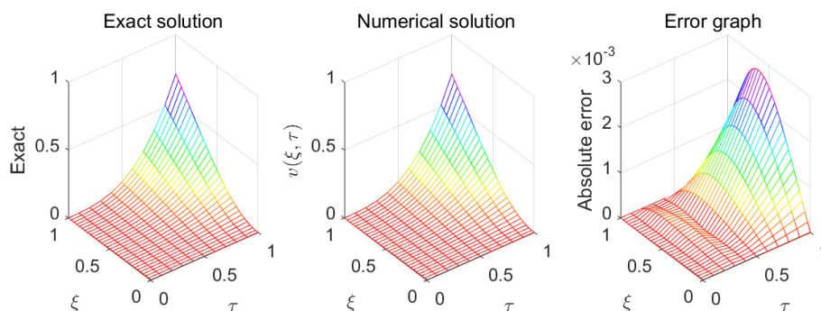
FIGURE 4. The 3D exact numerical \nu(\xi, \tau) and absolute error profile with \varsigma = 1.25 , \alpha = 1.5 , for M = 30 , \Delta\tau = 0.1 , and \tau \in [0, 1] for Example 6.1.
