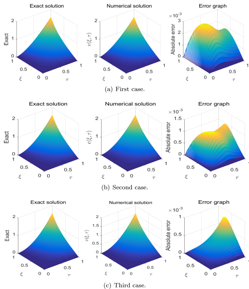
FIGURE 9. The 3D profile of exact numerical \mathcal{V}(\xi, \tau) and absolute error with \alpha = 1.95 , \tau \in [0, 1] .
