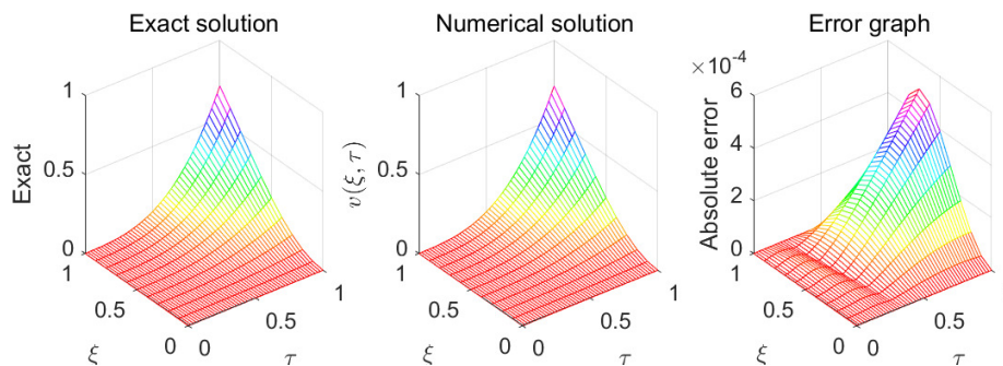
FIGURE 3. The 3D exact and numerical \nu(\xi, \tau) , and absolute error profile with \varsigma = 1.25 , \alpha = 1.5 , M = 10 , \Delta\tau = 0.02 , and \tau \in [0, 1] for Example 6.1.
