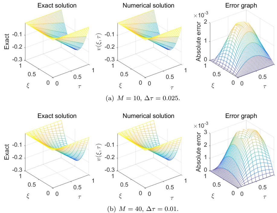
FIGURE 7. The 3D profile of exact numerical v(x, t) and absolute error for \alpha = 1.95 , \tau \in [0, 1] , with (a) M = 10 , \Delta\tau = 0.025 and (b) M = 40 , \Delta\tau = 0.01 for Example 6.2.
