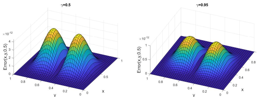
FIGURE 2. Plots of the absolute error function with values \vartheta = \nu = 1.75 , \alpha = 1.5 , and v = 0.1 when \mathcal{N} = 20 for Example 4.1.
