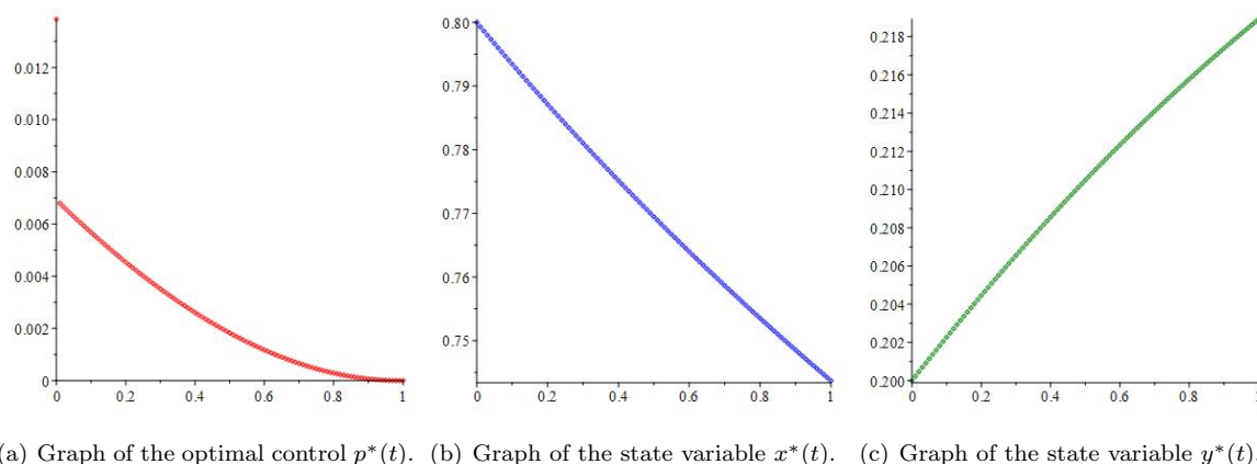
FIGURE 4. Optimal path diagrams.
