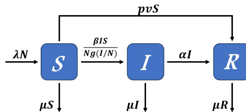
FIGURE 1. The diagram of SIR model (2.1).
