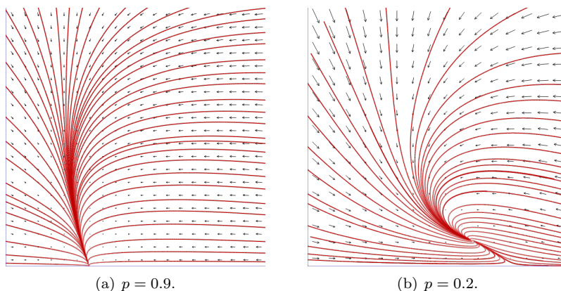
FIGURE 2. The phase portrait of system (3.1).
