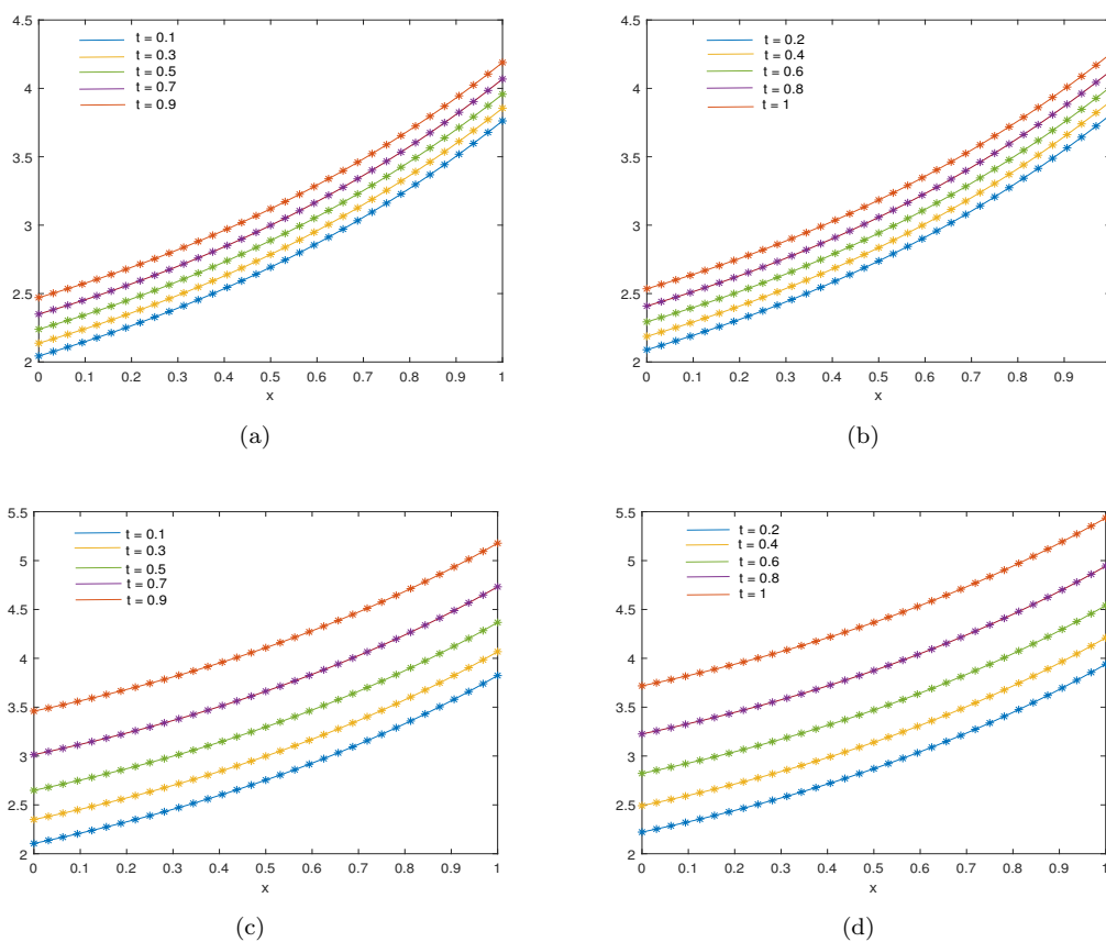
FIGURE 1. Approximate and exact solutions at different time points for Example 5.1 with k = 0.01 and M = 32 for (a) and (b) \gamma = 0.3 and (c) and (d) \gamma = 0.5 .
