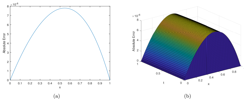
FIGURE 3. 2D and 3D error profiles respectively for Example 5.1 with k = 0.01 , \gamma = 0.5 , t = 1 , x \in [0, 1] and M = 90 .
