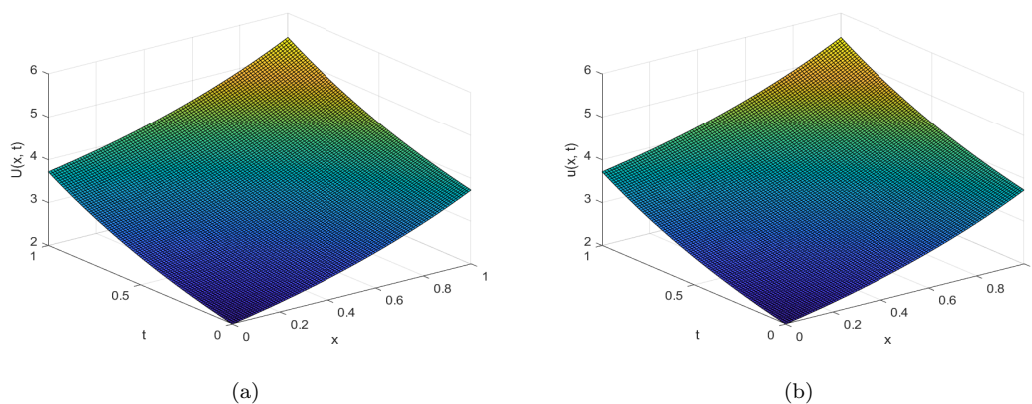
FIGURE 2. 3D approximate and exact solutions respectively for Example 5.1 with k = 0.01 , \gamma = 0.5 , t = 1 , x \in [0, 1] And M = 90 .
