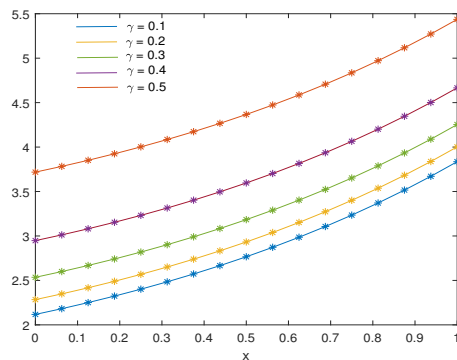
FIGURE 4. A comparison of the exact and approximate solutions at various \gamma values for Example 5.1, where k = 0.01 , t = 1 and M = 16 .
