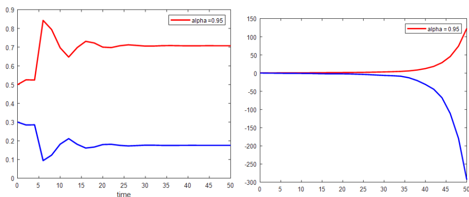
FIGURE 15. The comparison behavior of non-infected and infected cancer cells, between the fractional system (left) and the stochastic fractional system (right), for \alpha = 0.95 and parameter for disease state, that approximated using Newton's polynomial.
