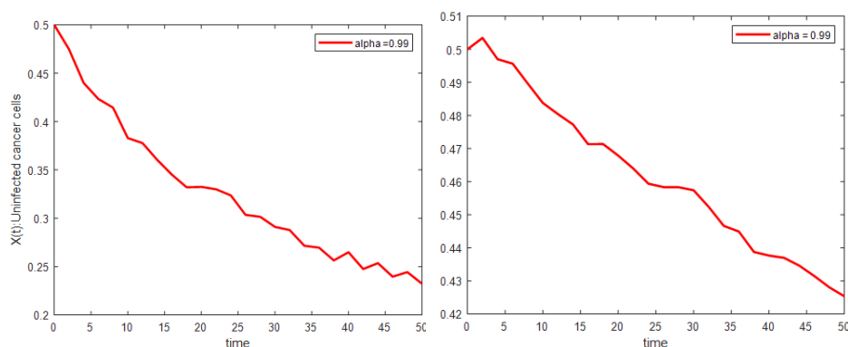
FIGURE 8. The comparison between the stochastic fractional system of x(t) , approximated using Lagrange's polynomial (left) and Newton's polynomial (right), for \alpha = 0.99 and parameter for disease state.
