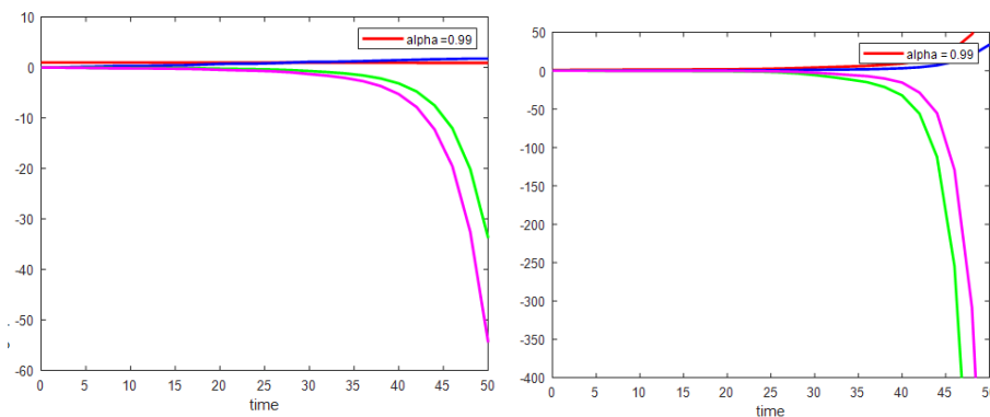
FIGURE 2. The simulations show the combined graphical behavior of subpopulations of cells in the stochastic fractional system (3.1) for \alpha=0.99 and parameter for E_0 . Left graph describes simulations approximated using Lagrange's polynomial, while right graph describes simulations approximated using Newton's polynomial.
