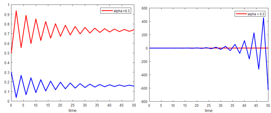
FIGURE 18. The comparison behavior of non-infected and infected cancer cells, between the fractional system (left) and the stochastic fractional system (right), for \alpha = 0.3 and parameter for disease state, that approximated using Lagrange's polynomial.
