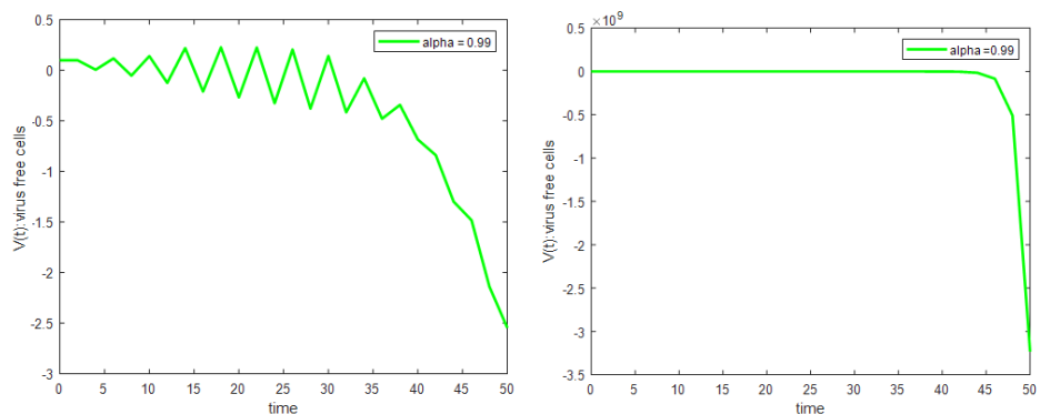
FIGURE 10. The comparison between the stochastic fractional system of v(t) , approximated using Lagrange's polynomial (left) and Newton's polynomial (right), for \alpha = 0.99 and parameter for disease state.
