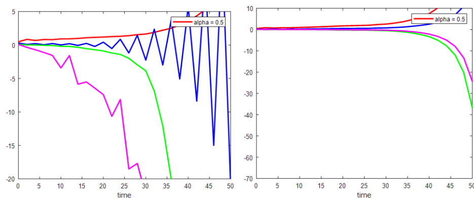
FIGURE 6. The simulations show the combined graphical behavior of subpopulations of cells in the stochastic fractional system (3.1) for \alpha=0.5 and the parameter for disease state. Left graph describes simulations approximated using Lagrange's polynomial, while right graph describes simulations approximated using Newton's polynomial.
