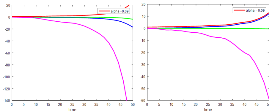
FIGURE 4. The simulations show the combined graphical behavior of subpopulations of cells in the stochastic fractional system (3.1) for \alpha = 0.09 and parameter for E_0 . Left graph describes simulations approximated using Lagrange's polynomial, while right graph describes simulations approximated using Newton's polynomial.
