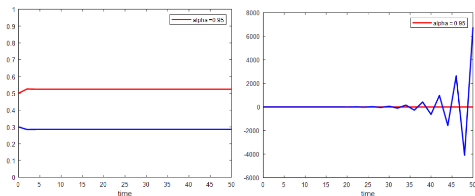
FIGURE 14. The comparison behavior of non-infected and infected cancer cells, between the fractional system (left) and the stochastic fractional system (right), for \alpha = 0.95 and parameter for disease state, that approximated using Lagrange's polynomial.
