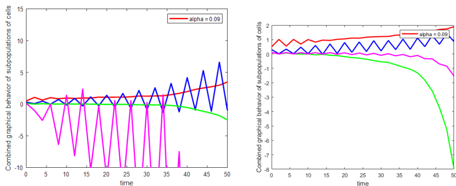
FIGURE 7. The simulations show the combined graphical behavior of subpopulations of cells in the stochastic fractional system (3.1) for \alpha=0.09 and the parameter for disease state. Left graph describes simulations approximated using Lagrange's polynomial, while right graph describes simulations approximated using Newton's polynomial.
