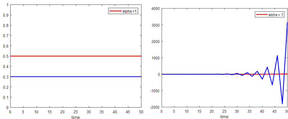
FIGURE 12. The comparison behavior of non-infected and infected cancer cells, between the ODE system and the stochastic differential system (SDE), for \alpha = 1 and parameter for disease state, that approximated using Lagrange's polynomial.
