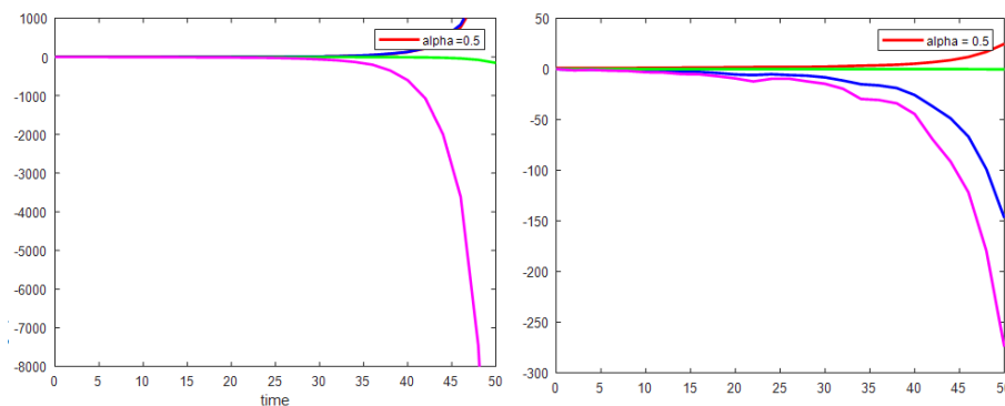
FIGURE 3. The simulations show the combined graphical behavior of subpopulations of cells in the stochastic fractional system (3.1) for \alpha=0.5 and parameter for E_0 . Left graph describes simulations approximated using Lagrange's polynomial, while right graph describes simulations approximated using Newton's polynomial.
