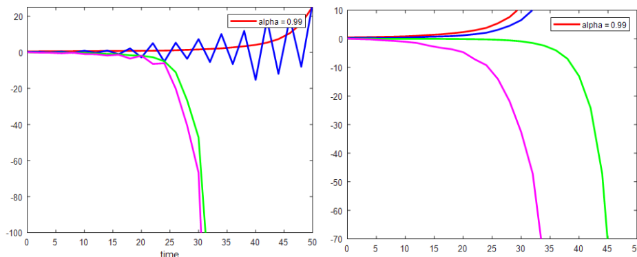
FIGURE 5. The simulations show the combined graphical behavior of subpopulations of cells in the stochastic fractional system (3.1) for \alpha = 0.99 and the parameter for disease state. Left graph describes simulations approximated using Lagrange's polynomial, while right graph describes simulations approximated using Newton's polynomial.
