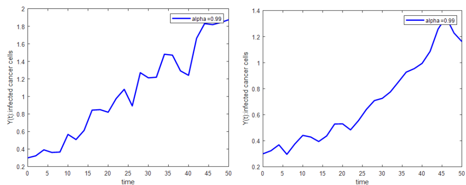
FIGURE 9. The comparison between the stochastic fractional system of y(t) , approximated using Lagrange's polynomial (left) and Newton's polynomial (right), for \alpha = 0.99 and parameter for disease state.
