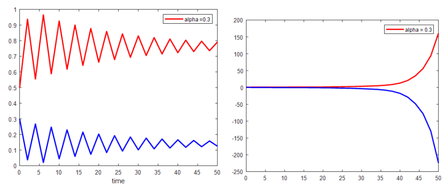
FIGURE 19. The comparison behavior of non-infected and infected cancer cells, between the fractional system (left) and the stochastic fractional system (right), for \alpha = 0.3 and parameter for disease state, that approximated using Newton's polynomial.
