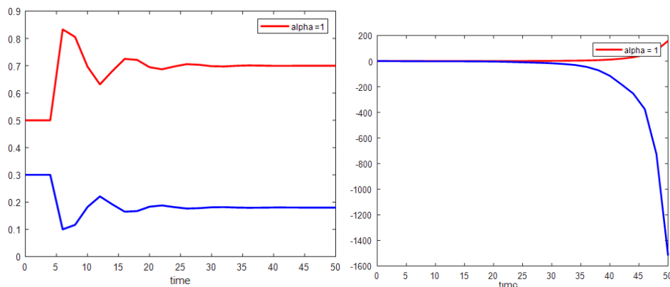
FIGURE 13. The comparison behavior of non-infected and infected cancer cells, between the ODE system and the stochastic differential system (SDE), for \alpha = 1 and parameter for disease state, that approximated using Newton's polynomial.
