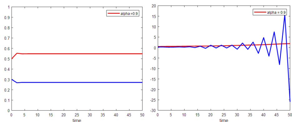
FIGURE 16. The comparison behavior of non-infected and infected cancer cells, between the fractional system (left) and the stochastic fractional system (right), for \alpha = 0.9 and parameter for disease state, that approximated using Lagrange's polynomial.
