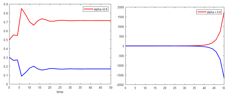
FIGURE 17. The comparison behavior of non-infected and infected cancer cells, between the fractional system (left) and the stochastic fractional system (right), for \alpha = 0.9 and parameter for disease state, that approximated using Newton's polynomial.
