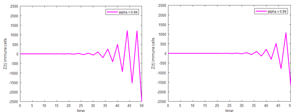
FIGURE 11. The comparison between the stochastic fractional system of z(t) , approximated using Lagrange's polynomial (left) and Newton's polynomial (right), for \alpha = 0.99 and parameter for disease state.
