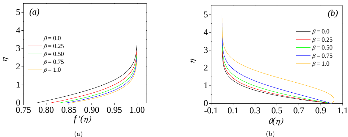
FIGURE 4. Variation of velocity and thermal profiles for different \beta at K = 0.25 , Pr = 1 , N = 1.5 , \lambda = 0.5 .
