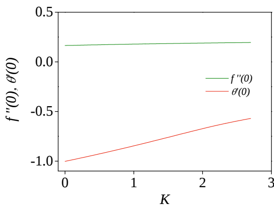
FIGURE 6. Variation of wall shear stress ( f''(0) ) and Nusselt number ( \theta'(0) ) values as a function of unsteady parameter K for Pr = 1 , \beta = 0.5 , N = 1 , \lambda = 0.7 .
