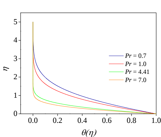
FIGURE 5. Variation of temperature for different values of Prandtl number Pr at K = 0.25 , \beta = 0.5 , N = 1.5 , \lambda = 0.5 .
