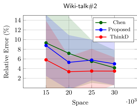
FIGURE 3. Comparison (edge-arrival) on Wiki-talk dataset.
