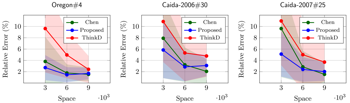
FIGURE 1. Comparison of algorithms (edge-arrival) on Oregon and CAIDA datasets.
