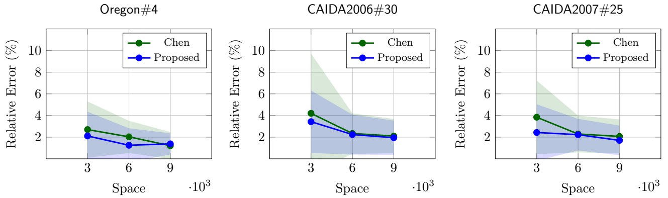
FIGURE 4. Comparison (vertex-arrival) OREGON and CAIDA datasets.
