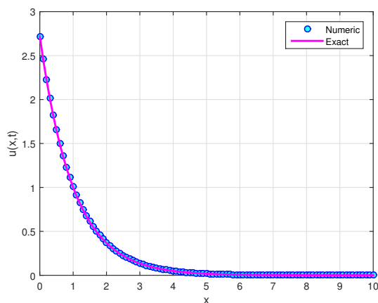
(c) h = 0.1 and k = 0.5 .
