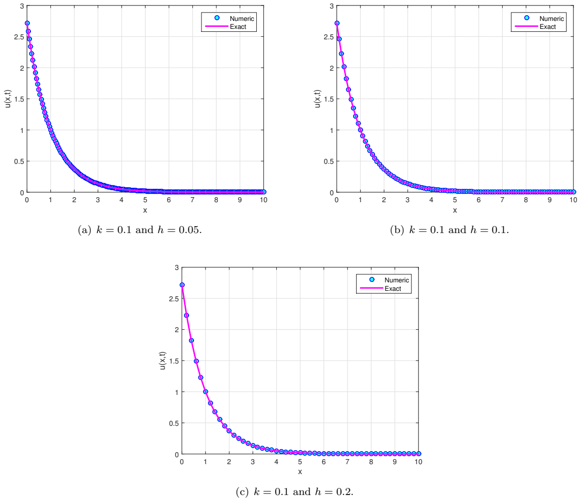
FIGURE 2. Numerical solution and exact solution of the CDF with k = 0.1 and h = 0.05 , k = 0.1 and h = 0.2 at time t = 1 .
