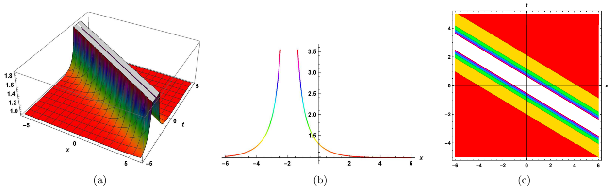
FIGURE 4. The 3D, 2D and contour plots of q_4(x, t) in (4.9) is generated for used values are \alpha = 0.1, \beta = 2.2, v = 1, c = 0.5, y = -0.2, \lambda = -1, \varepsilon = 1 . Also, -6 \leq x \leq 6 and -5 \leq t \leq 5 .
