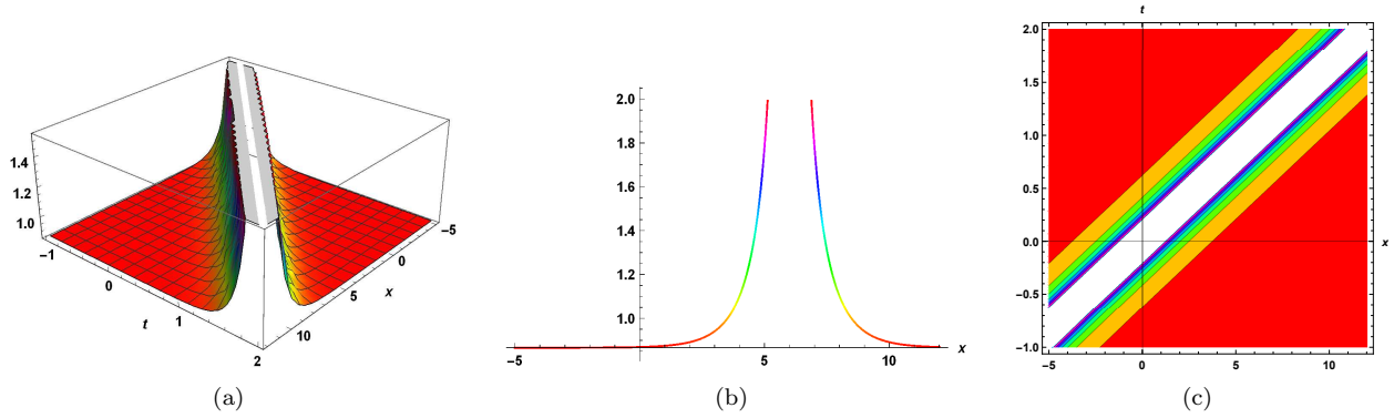
FIGURE 2. The 3D, 2D and contour plots of q_6(x, t) in (3.12) is generated for used values are \alpha = 3, v = 2, \lambda = -1, \varepsilon = 1 . Also, -5 \leq x \leq 12 and -1 \leq t \leq 2 .
