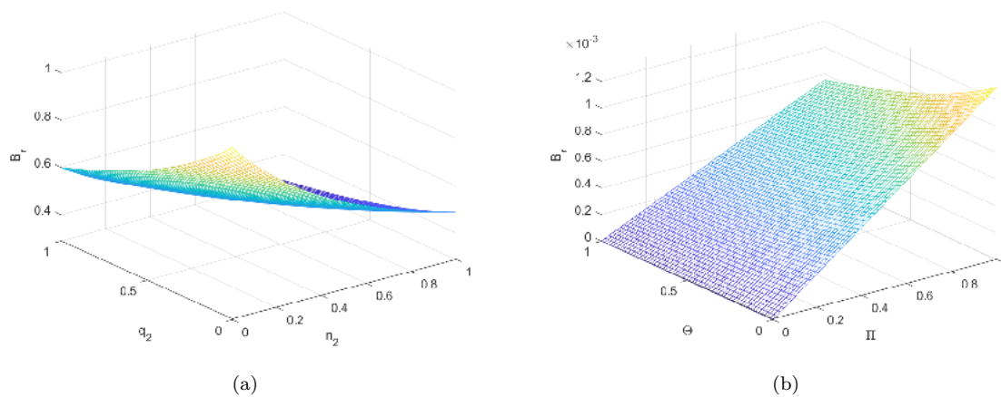
FIGURE 2. (a) Behaviour of B_r against q_2 and n_2 , (b) Behaviour of B_r against \Theta and \Pi .
