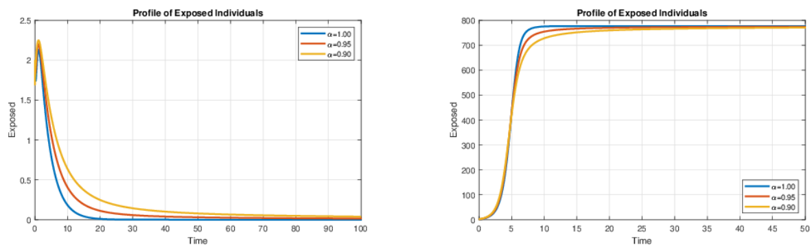
FIGURE 9. Numerical solutions of system (4.1) utilizing fractional order ABC derivative, with \mathcal{E}_f = 0 and \mathcal{E}_p = 776.6 . Left: The exposed profile \mathcal{E}(t) for D_f is depicted on the left side, employing the ABC fractional derivative, while the exposed profile \mathcal{E}(t) for D_p is presented on the right side using the ABC fractional derivative.
