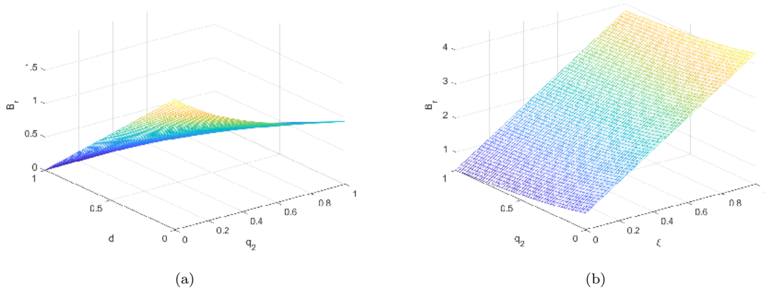
FIGURE 4. (a) Behaviour of B_r against d and q_2 , (b) Behaviour of B_r against q_2 and \xi .
