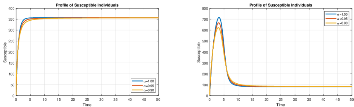
FIGURE 8. Numerical solutions of the system (4.1) using fractional order ABC derivative with \mathcal{S}_f = 357.1429 , \mathcal{S}_p = 81.89 . Left: The susceptible profile \mathcal{S}(t) for D_f is shown on the left side using the ABC fractional derivative, while the susceptible profile \mathcal{S}(t) for D_p is displayed on the right side using the ABC fractional derivative.
