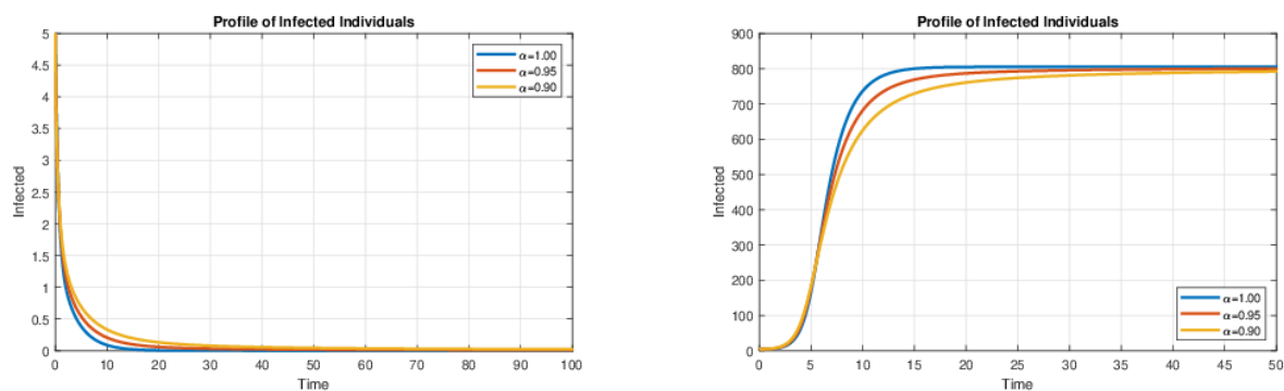
FIGURE 10. Numeric solutions for system (4.1) are obtained using a fractional order ABC derivative with \mathcal{I}_f = 0 and \mathcal{I}_p = 804.9 . On the left, the infected profile \mathcal{I}(t) for D_f is shown utilizing the ABC fractional derivative, while on the right, the infected profile \mathcal{I}(t) for D_p is depicted using the ABC fractional derivative.
