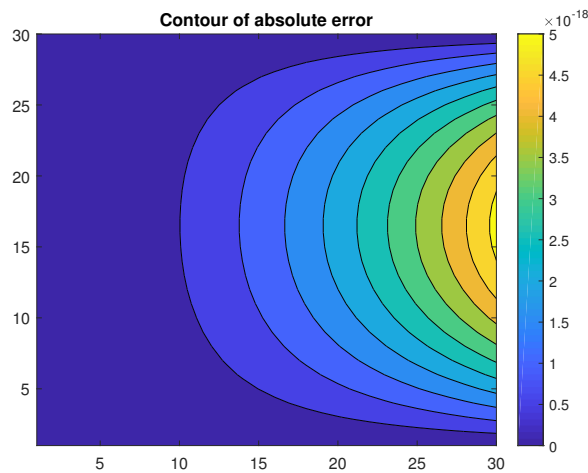
FIGURE 8. Contour plot of the maximum absolute error of instance 4.
