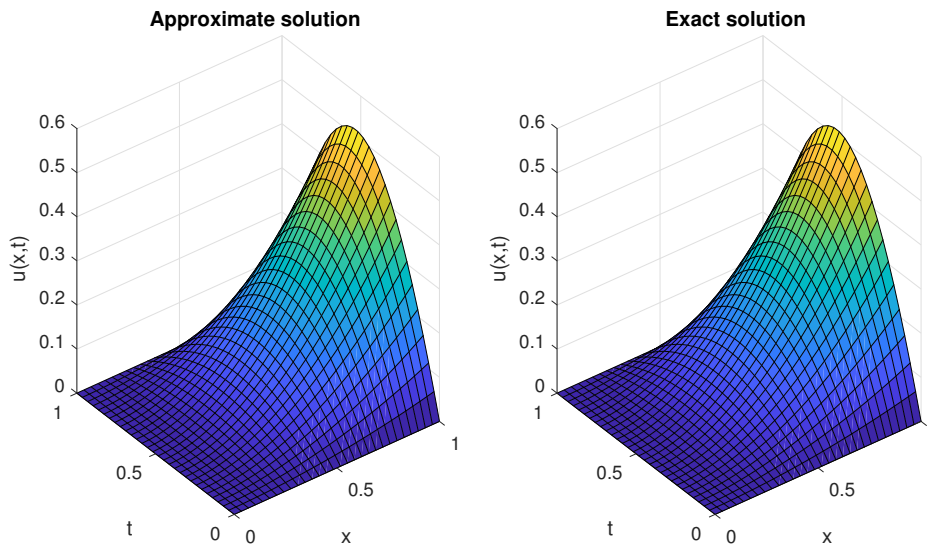
FIGURE 7. Plot of the analytical and approximate solutions of instance 4.
