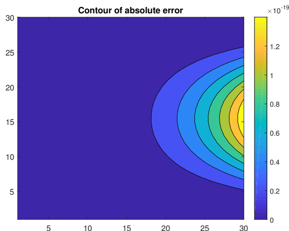
FIGURE 2. Contour plot of absolute error of Example 3.1.
