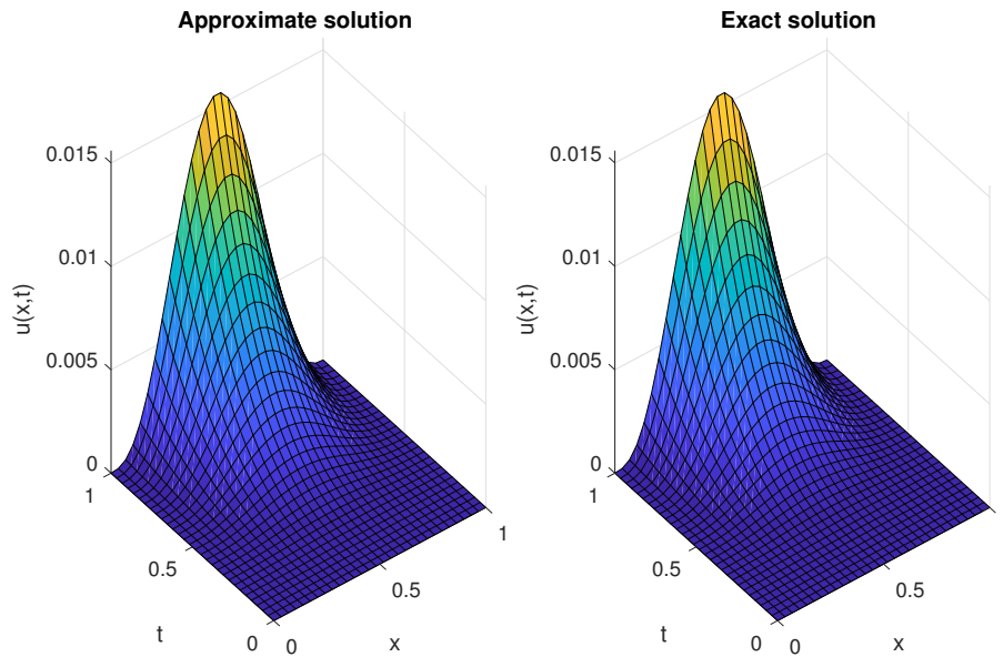
FIGURE 1. Plot of the analytical and approximate solutions of Example 3.1.
