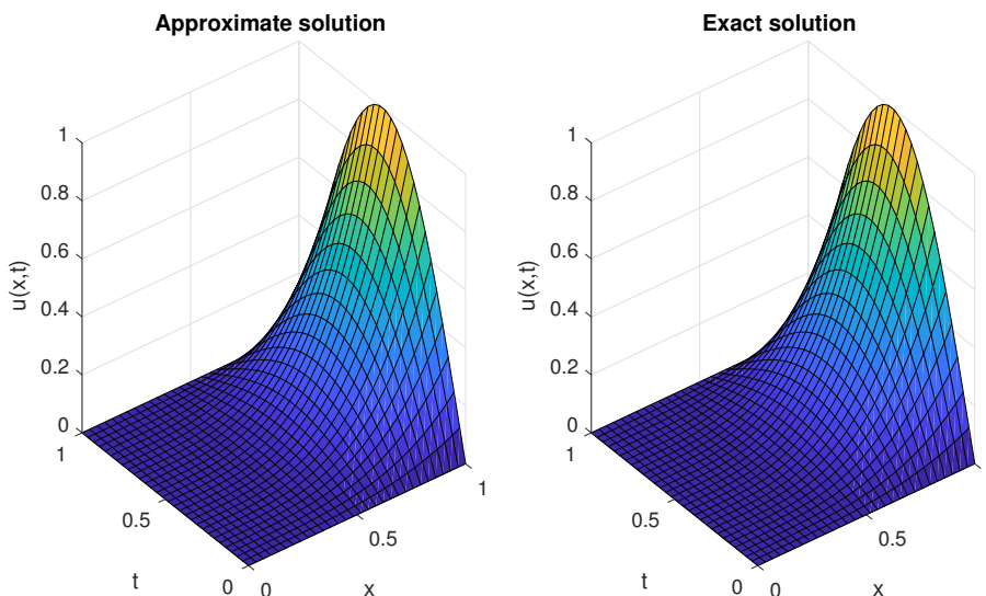
FIGURE 5. Plot of the analytical and approximate solutions of instance 3.
