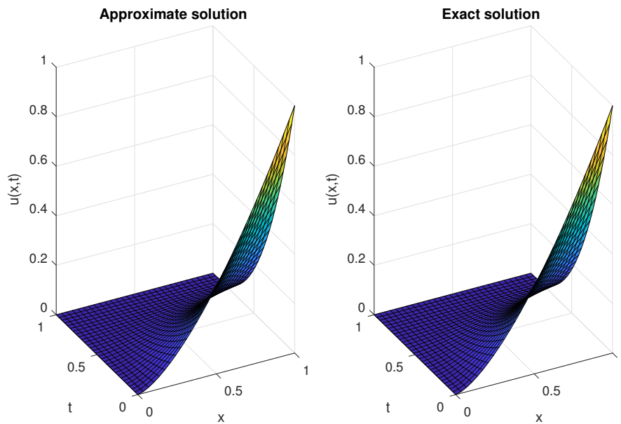
FIGURE 3. Plot of the analytical and approximate solutions of Example 3.2.
