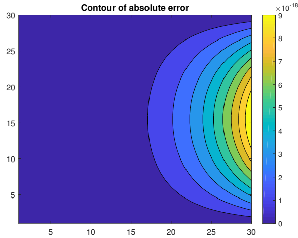
FIGURE 6. Contour plot of the maximum absolute error of instance 3.
