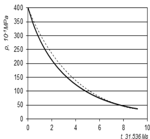
FIGURE 2. Dynamics of reservoir pressures in cases where heterogeneity is taken into account (solid line) and neglected (dashed line).
