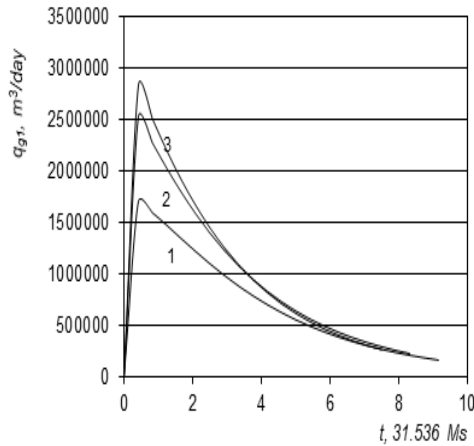
FIGURE 6. Dynamics of the curves of gas flow flowing from the external zone to the internal zone at different values of R_e/r_k : 1-1.5, 2-5 and 3-10.
