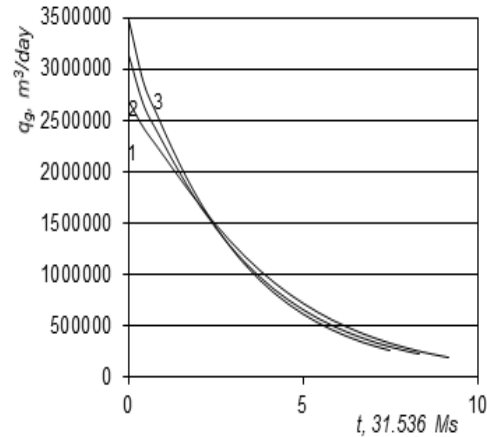
FIGURE 7. Dynamics of well flow rate at different values of R_e/r_k : 1-1.5, 2-5 and 3-10.
