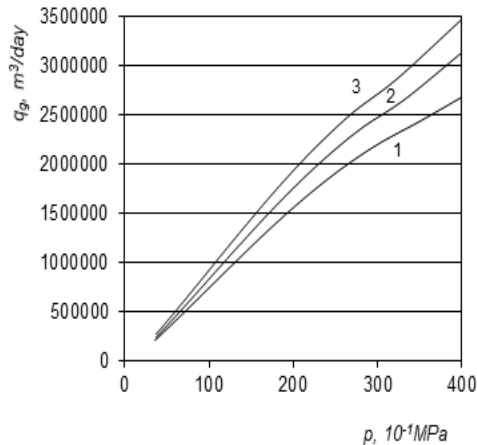
FIGURE 5. Dependency curves of gas flow rate in a rheologically heterogeneous formation at various values of R_e/r_k : 1-1.5, 2-5 and 3-10.
