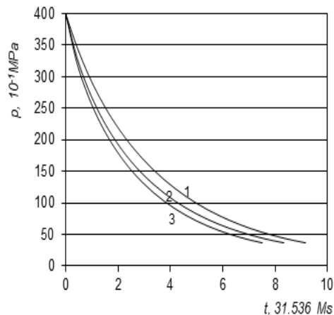
FIGURE 4. Dynamics of the reservoir pressure in a rheologically heterogeneous formation at different values of R_e/r_k : 1-1.5, 2-5 and 3-10.
