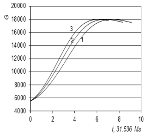
FIGURE 9. Dynamics of the gas condensate factor at various values of R_e/r_k : 1-1.5, 2-5 and 3-10.
