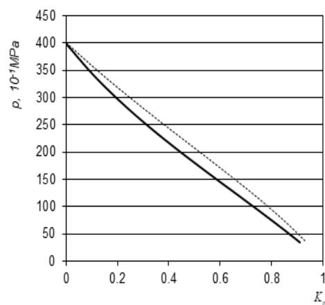
FIGURE 3. Dependence of reservoir pressures on the gas recovery factor in heterogeneous (solid line) and homogeneous reservoirs (dashed line).
