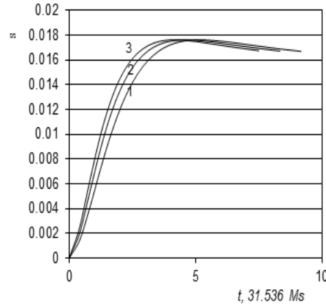
FIGURE 8. Dynamics of the condensate saturation coefficient at different values of R_e/r_k : 1-1.5, 2-5 and 3-10.
