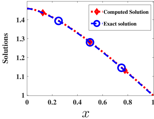
(A) Solutions for \alpha = 1.4 , \beta = 0.8 , N = 256 .
