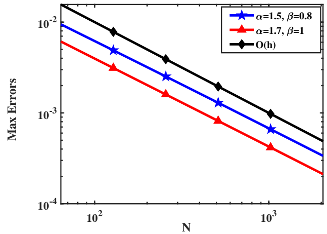
(B) Log-log plots for various values of \alpha and \beta .
