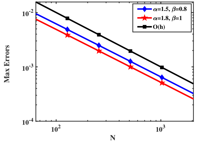
(B) Log-log plot for various values of \alpha and \beta .
