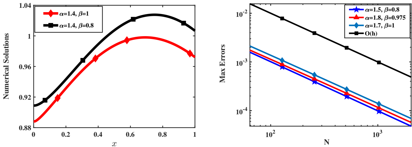
(A) Numerical solutions of Example 6.2 for N = 128 .
