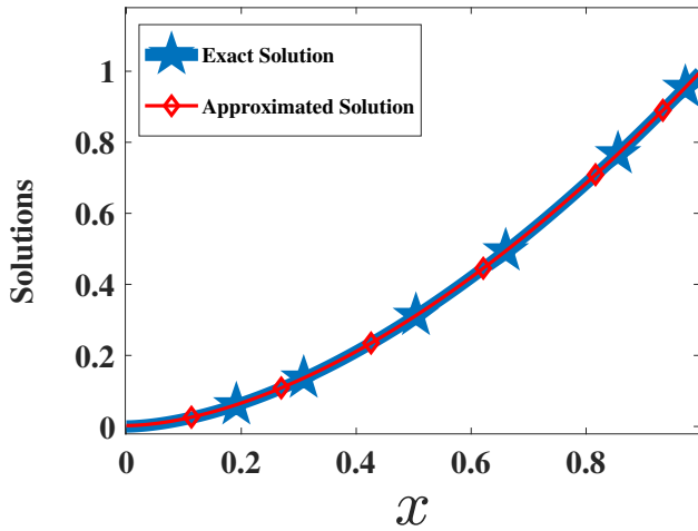
(A) Solutions for \alpha = 1.5 , \beta = 0.8 and N = 256
