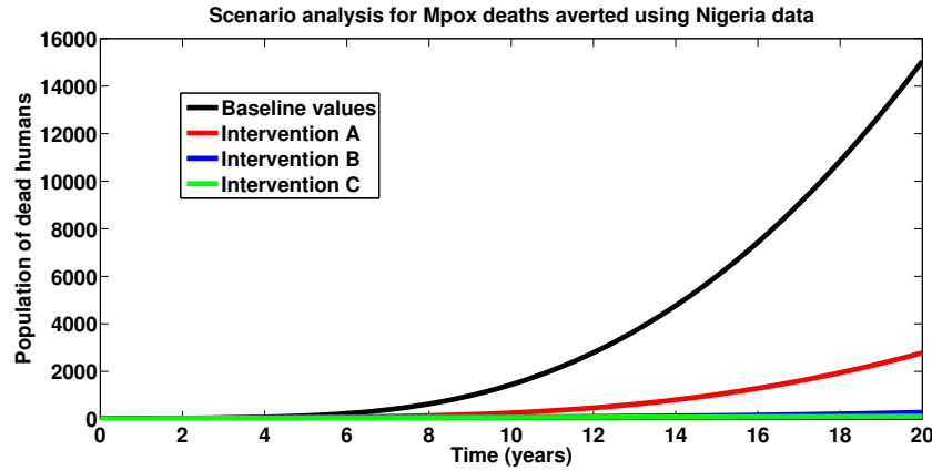
FIGURE 11. Scenario analysis for Mpox deaths averted using Nigeria data. Here, Baseline values: \alpha_h = 0.5712 , \alpha_r = 0.8489 , \tau = 0.0066 ; Intervention A: \alpha_h = 0.3 , \alpha_r = 0.5 , \tau = 0.003 ; Intervention B: \alpha_h = 0.1 , \alpha_r = 0.25 , \tau = 0.001 ; Intervention C: \alpha_h = 0.05 , \alpha_r = 0.15 , \tau = 0.0005 .
