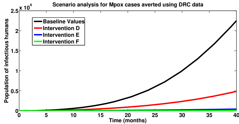
FIGURE 13. Scenario analysis for Mpox cases averted using DRC data. Here, Baseline values: \alpha_h = 0.1005 , \alpha_r = 0.1284 , \tau = 0.0428 ; Intervention D: \alpha_h = 0.05 , \alpha_r = 0.08 , \tau = 0.03 ; Intervention E: \alpha_h = 0.025 , \alpha_r = 0.04 , \tau = 0.01 ; Intervention F: \alpha_h = 0.010 , \alpha_r = 0.02 , \tau = 0.0005 .
