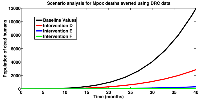
FIGURE 15. Scenario analysis for Mpox deaths averted using DRC data. Here, Baseline values: \alpha_h = 0.1005 , \alpha_r = 0.1284 , \tau = 0.0428 ; Intervention D: \alpha_h = 0.05 , \alpha_r = 0.08 , \tau = 0.03 ; Intervention E: \alpha_h = 0.025 , \alpha_r = 0.04 , \tau = 0.01 ; Intervention F: \alpha_h = 0.010 , \alpha_r = 0.02 , \tau = 0.0005 .
