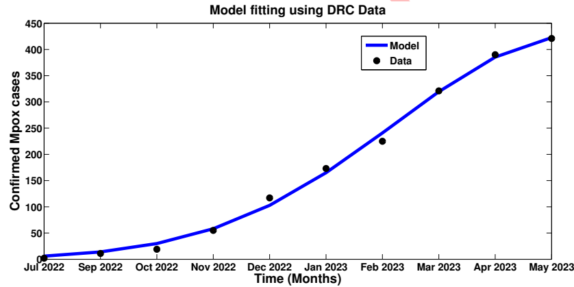
FIGURE 4. Fitting of the model to the Confirmed Mpox cases For Democratic Republic of Congo (DRC).
