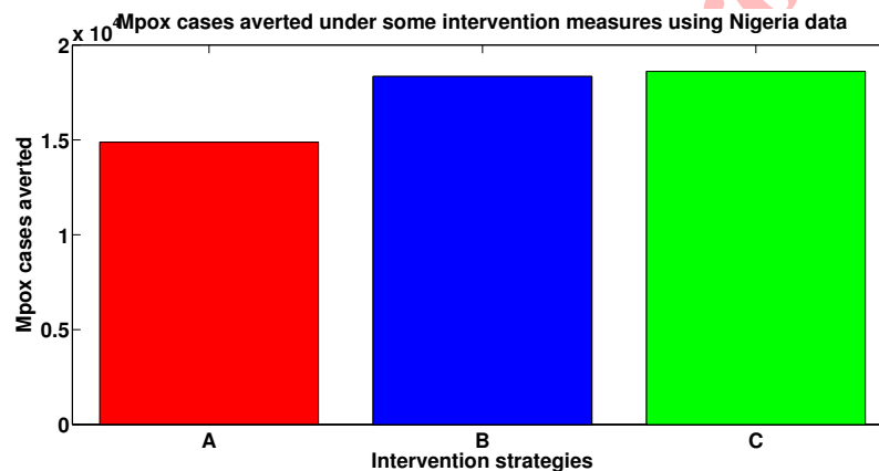
FIGURE 10. Mpox cases averted under different intervention measures using Nigeria data.
