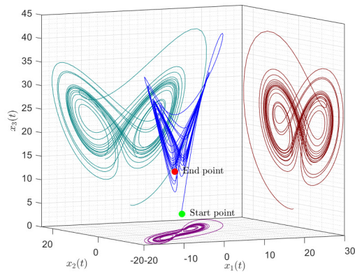
FIGURE 4. 3D Trajectory of FCFS Attractor with Shadow Projections on Planes.
