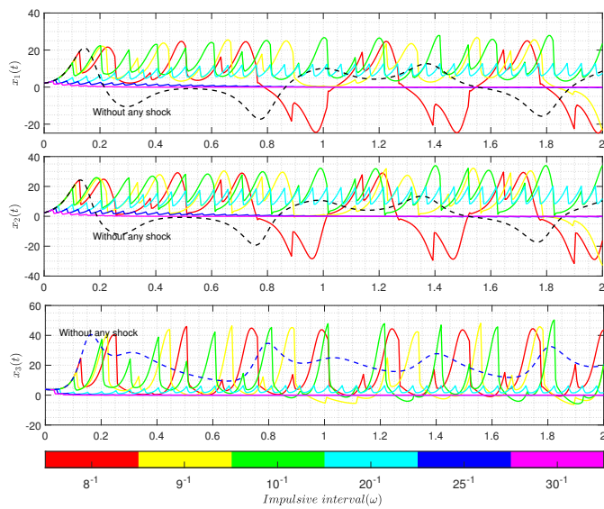
FIGURE 5. Numerical computation of fractional impulsive system results employing the proposed approach across various impulsive intervals, with \varrho_1 = 0.93 , \varrho_2 = 0.98 , \varrho_3 = 0.85 , and \delta = 0.005 .
