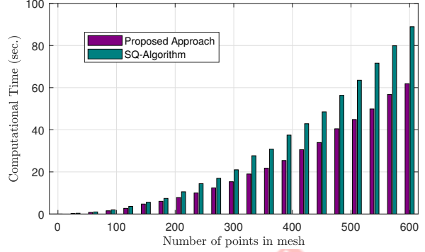
FIGURE 2. Comparative computational times of Proposed Approach and SQ-Algorithm [31] across mesh resolutions with \varrho = 0.95 .
