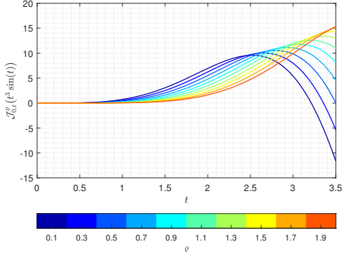
FIGURE 1. Impact of \varrho on the dynamics of \mathcal{J}_{0,t}^{\varrho}(t^3 \sin(t)) using the Proposed Approach with \delta = 0.01 .
