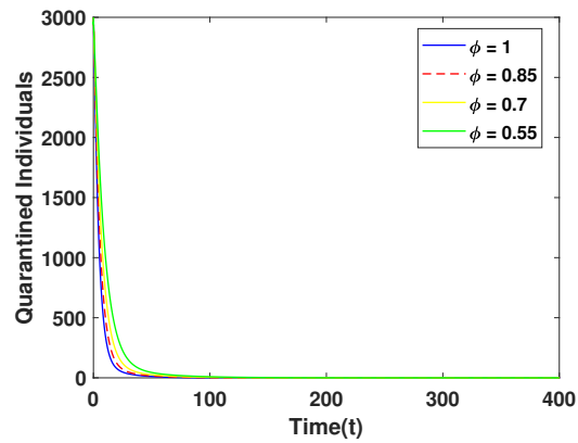
FIGURE 6. Quarantined Individuals versus time.
