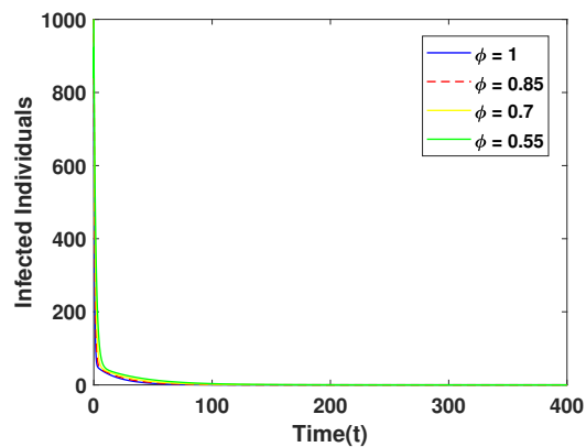
FIGURE 5. Infected Individuals versus time.
