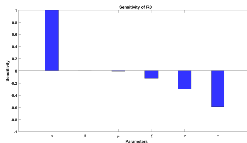
FIGURE 2. Sensitivity indices of parameters.
