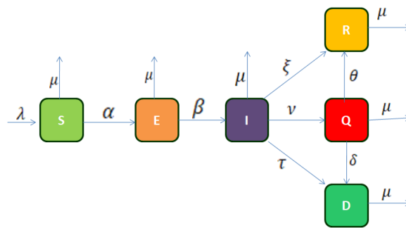
FIGURE 1. Schematic diagram of the SEIQRD model.
