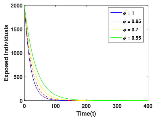
FIGURE 4. Exposed individuals versus time.
