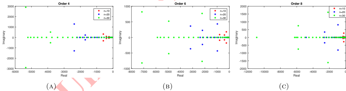
FIGURE 2. The eigenvalues of coefficient matrix by the proposed method for the case m = 0 in Example 4.2.
